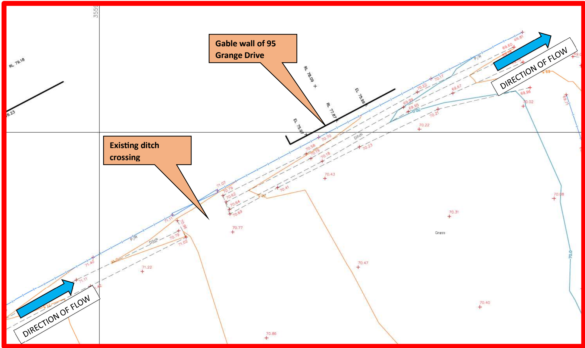
A topographical survey drawing of the site was submitted as part of outline application referene no. 20/01399/OUTMAJ and shows the existing ditch system along the northern boundary of the site upstream of where it connects in to Tanyard Brook.
